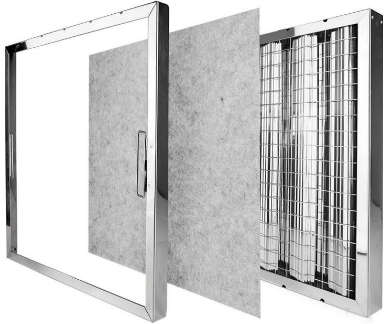
Stainless Steel #403 Baffle Filter Frame with Wool - 495 X 495mm
